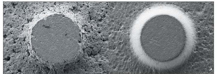
Conventional vs newly developed manufacturing process for burls.
