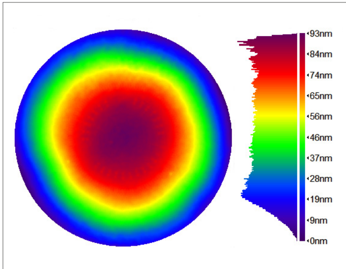
Flatness profile - interferometric image.
